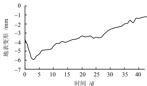
图 6 融沉注浆期间通道中部地表变形曲线 Fig.6 Ground settlement above the middle of connected aisle during thaw settlement grouting construction
