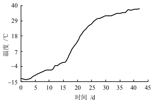
图 5 强制解冻期间 C5 孔温度变化曲线 Fig.5 Curve of temperature in C5 monitoring hole during forced thaw period
